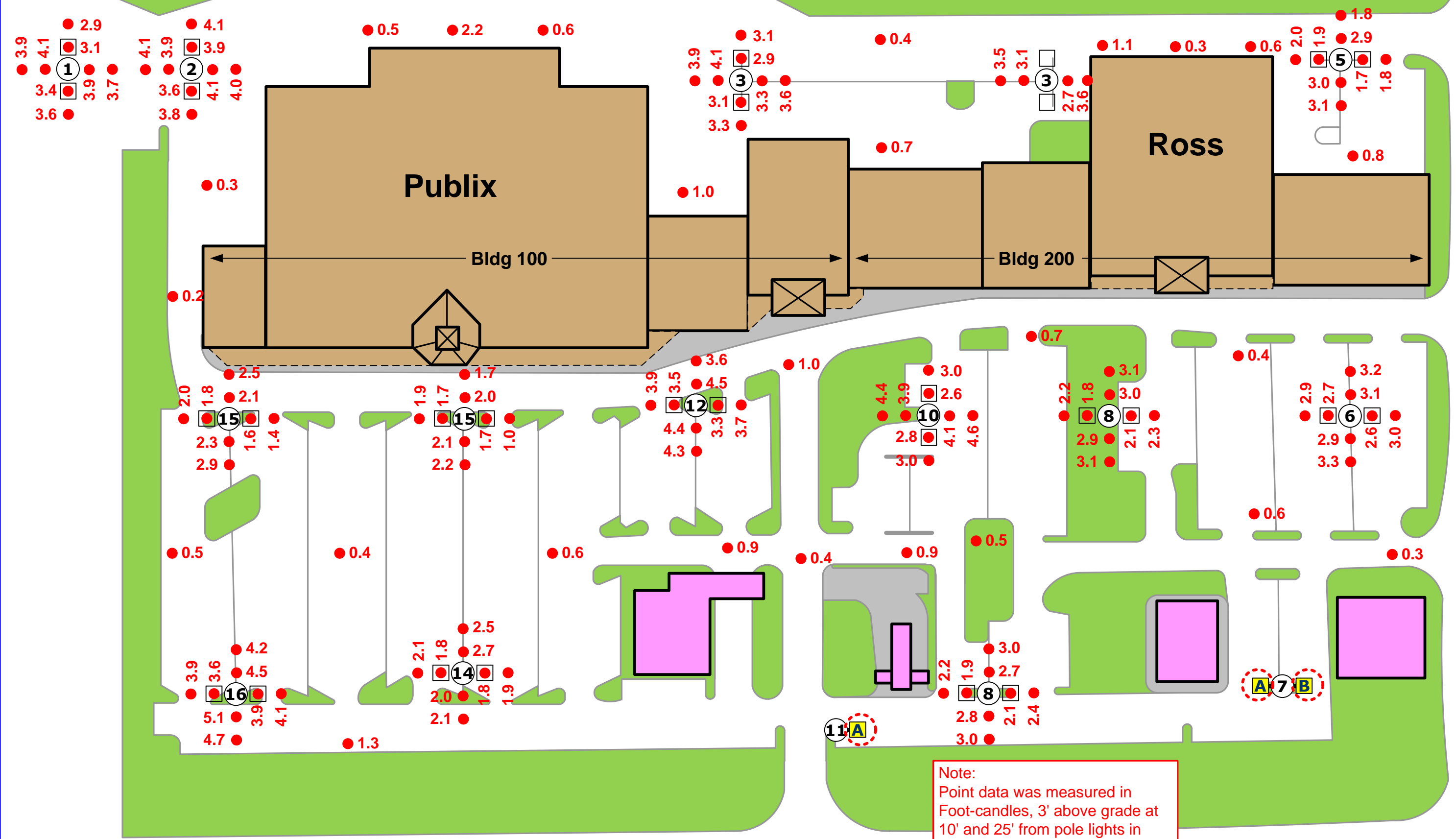
Photometric Survey
